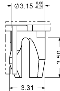
DETAIL B Scale 4 : 1
