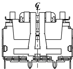
RIGHT VIEW
